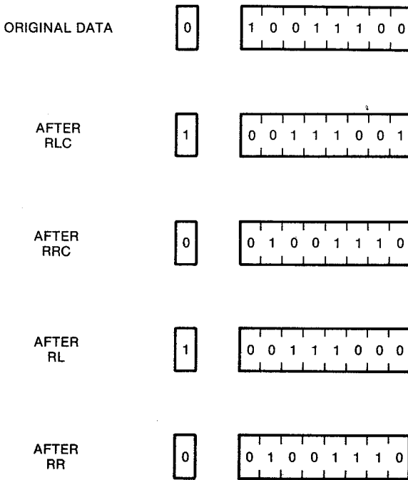
Fig. 12-3. Typical results of the ROTATE operations.
